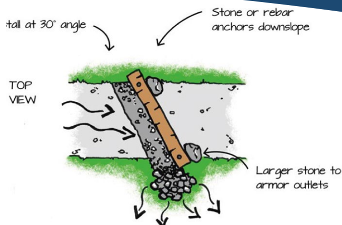
Plan view of water bar at angle with stone outlet.
