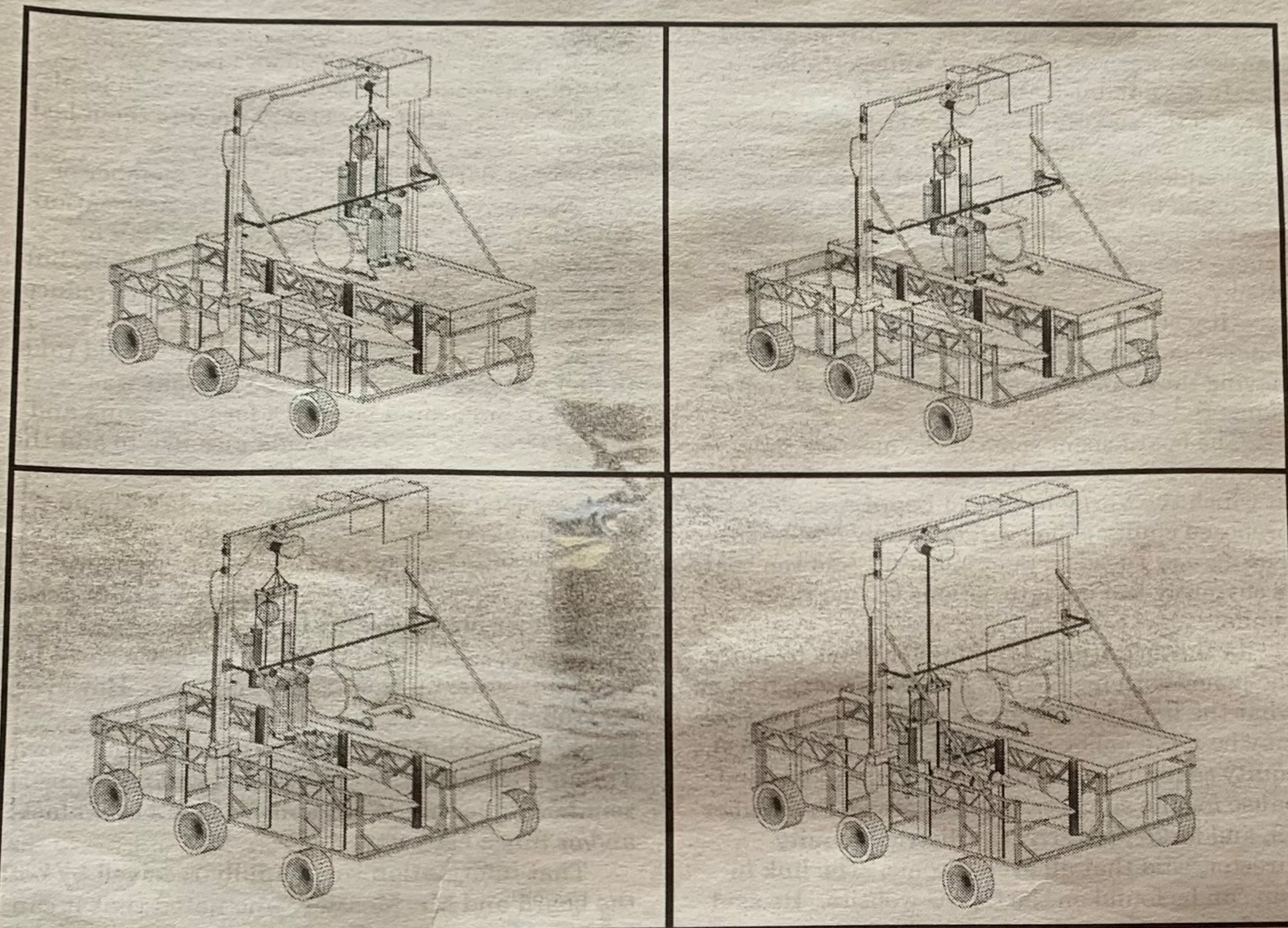
A series of diagrams demonstrate the lift's function. The user sits in the harness on the dock. The lift raises the user. The user then pulls on the guidebar, until above the kayak. The lift then lowers the user into the kayak.
